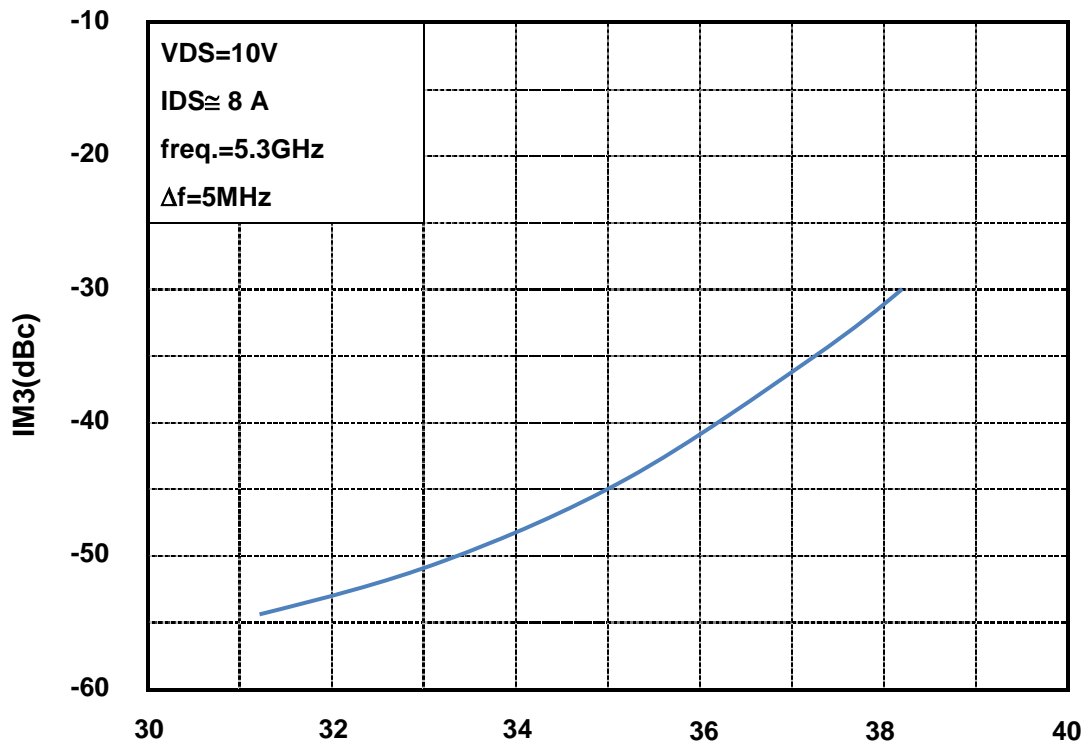
IM3 vs. Output Power Characteristics
