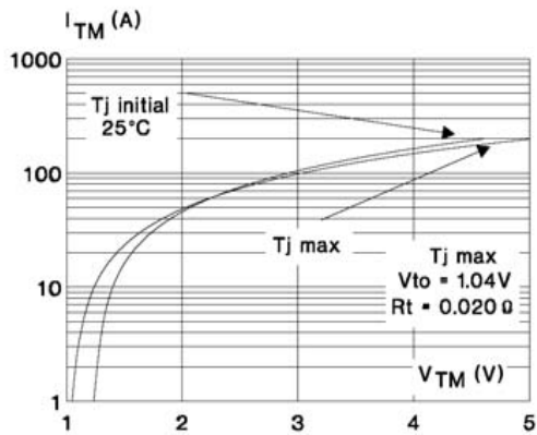
Fig. 9: On-state characteristics (maximum values).
