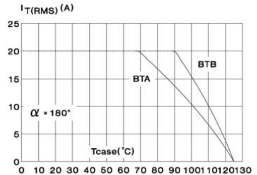
Fig. 4: RMS on-state current versus case temperature.
