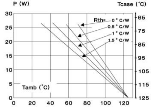
Fig. 2: Correlation between maximum RMS power dissipation and maximum allowable temperatures ( T_{amb} and T_{case} ) for different thermal resistances heatsink + contact (BTA).
