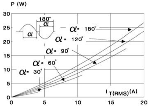
Fig. 1: Maximum RMS power dissipation versus RMS on-state current ( F = 50\text{Hz} ). (Curves are cut off by (di/dt)_c limitation)
