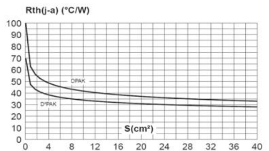
Fig. 10: DPAK and D 2 PAK Thermal resistance junction to ambient versus copper surface under tab (printed circuit board FR4, copper thickness: 35 µm).
