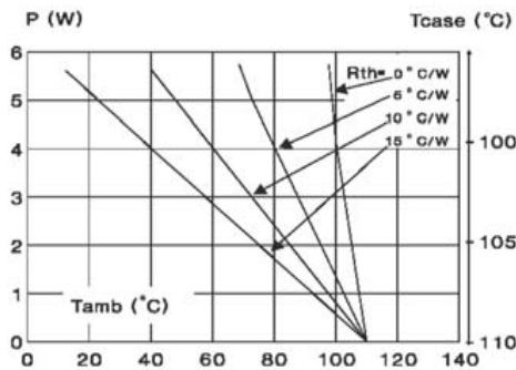
Fig. 3: Correlation between maximum RMS power dissipation and maximum allowable temperature ( T_{amb} and T_{case} ) for different thermal resistances heatsink + contact (BTB).
