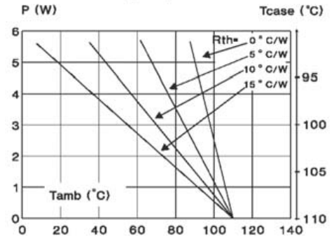
Fig. 2: Correlation between maximum RMS power dissipation and maximum allowable temperature ( T_{amb} and T_{case} ) for different thermal resistances heatsink + contact (BTA).
