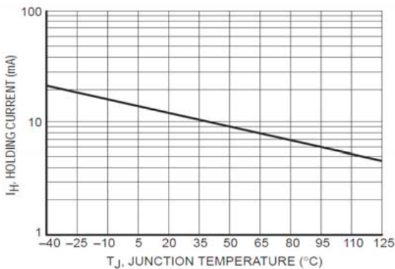
Figure 5. Typical Holding Current versus Junction Temperature
