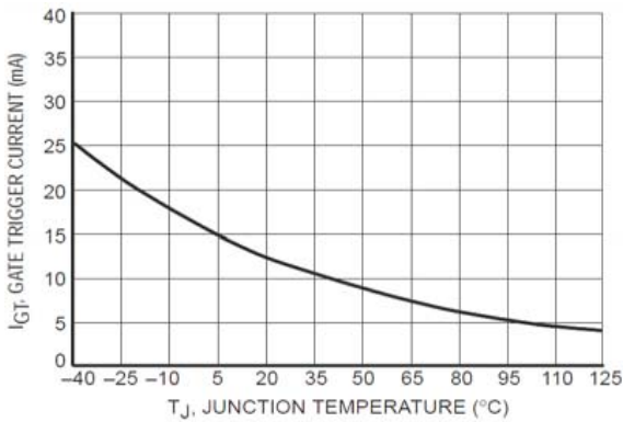
Figure 1. Typical Gate Trigger Current versus Junction Temperature
