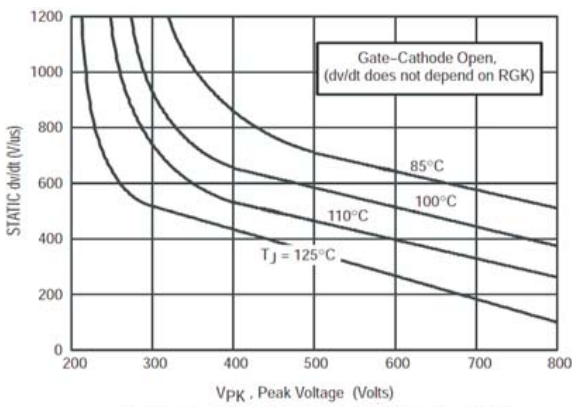
Figure 9. Typical Exponential Static dv/dt Versus Peak Voltage.
