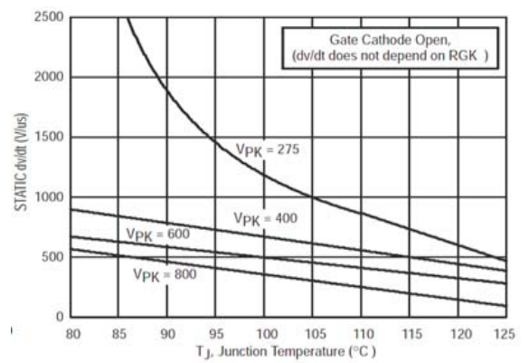
Figure 10. Typical Exponential Static dv/dt Versus Junction Temperature.
