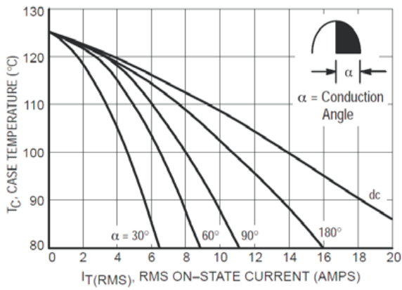
Figure 7. Typical RMS Current Derating
