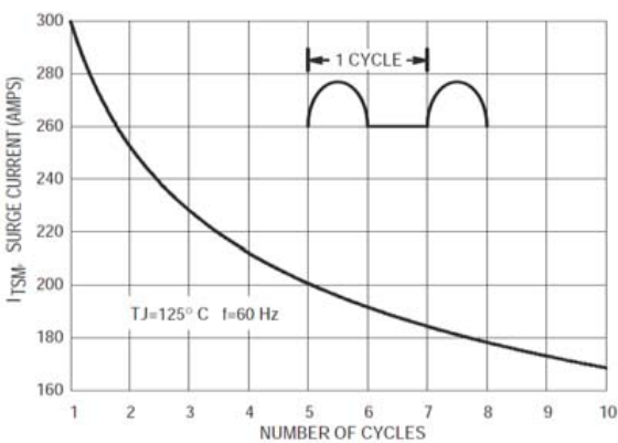
Figure 11. Maximum Non-Repertive Surge Current
