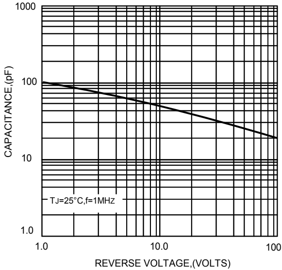
FIG.3-TYPICAL JUNCTION CAPACITANCE
