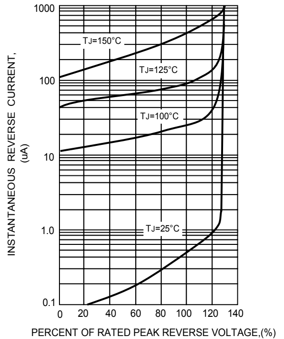
FIG.5-TYPICAL REVERSE CHARACTERISTICS
