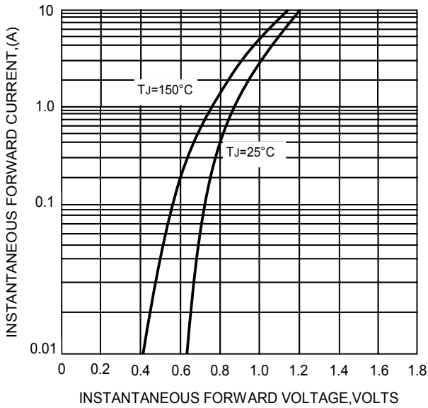
FIG.4-TYPICAL FORWARD CHARACTERISTICS
