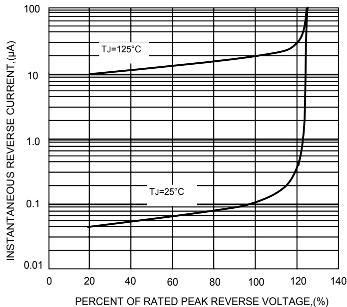
FIG.5-TYPICAL REVERSE CHARACTERISTICS
