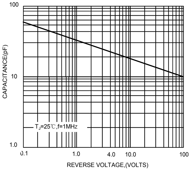
FIG.3-TYPICAL JUNCTION CAPACITANCE
