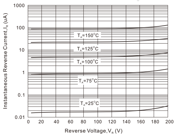
Fig. 3 - Reverse Characteristics
