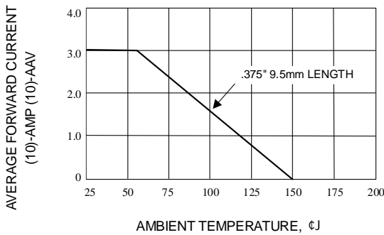
Fig. 2-FORWARD CURRENT CURVE
