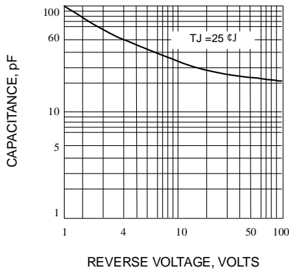
Fig. 4-TYPICAL JUNCTION CAPACITANCE
