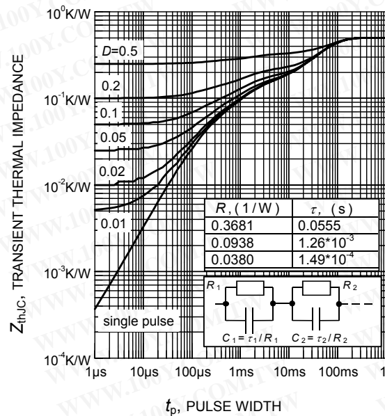
Figure 16. IGBT transient thermal impedance as a function of pulse width ( D = t_p / T )
