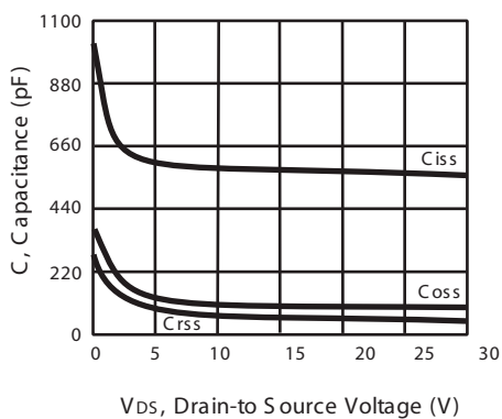
Figure 3. Capacitance
