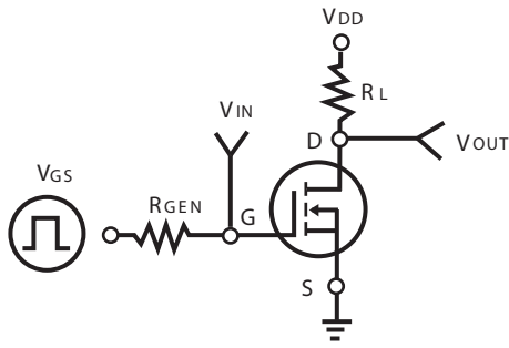
Figure 11. S Switching Test Circuit
