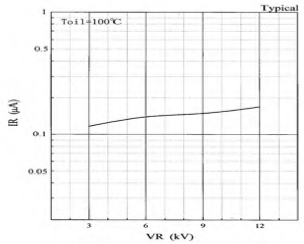
Fig. 2 Reverse characteristic [VR-IR]
