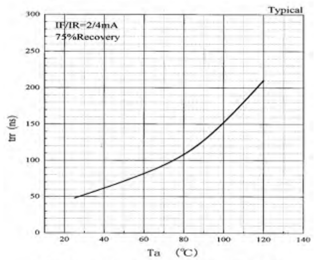
Fig. 4 Reverse recovery time characteristic [Ta-trr]
