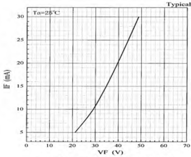
Fig. 1 Forward characteristic [VF-IF]
