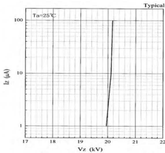
Fig. 3 Avalanche characteristic [Vz-Iz]
