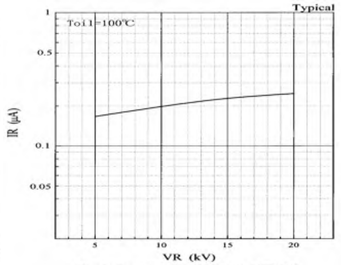
Fig. 2 Reverse characteristic [VR-IR]
