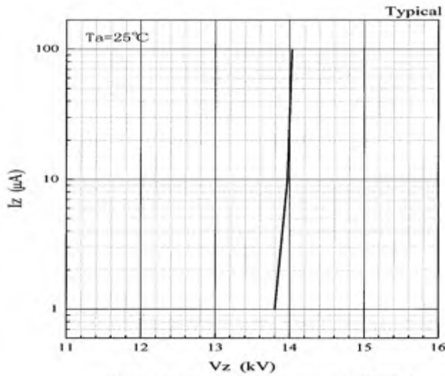
Fig. 3 Avalanche characteristic [Vz-Iz]
