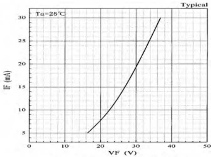
Fig. 1 Forward characteristic [VF-IF]
