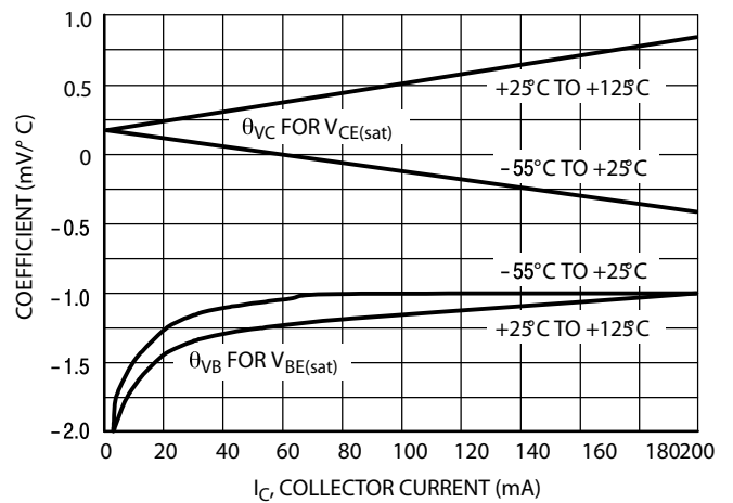
Figure 20. Temperature Coefficients
