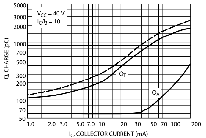
Figure 4. Charge Data
