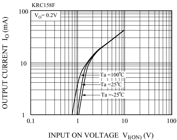
I_O - V_{I(ON)}
