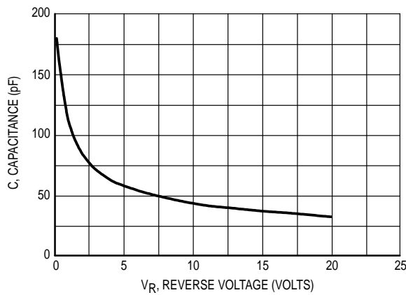
Figure 3. Typical Capacitance
