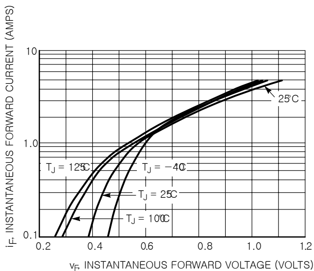
Figure 1. Typical Forward Voltage
