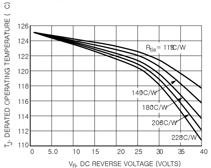
Figure 8. Typical Operating Temperature Derating*
