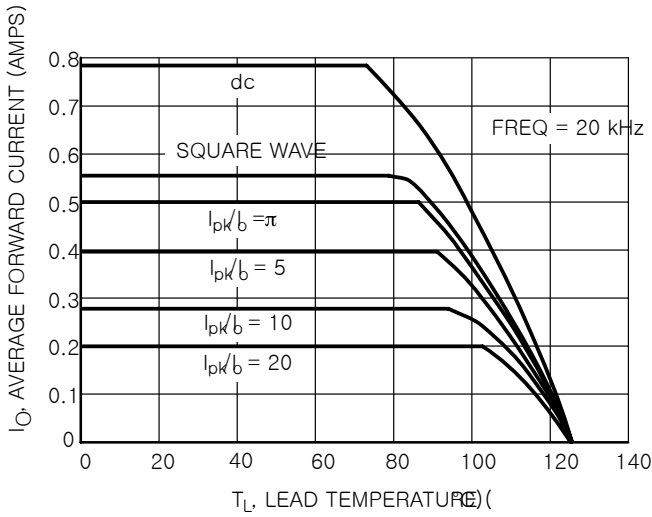
Figure 5. Current Derating
