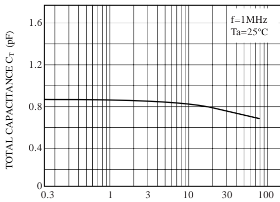
Fig.3 REVERSE VOLTAGE V R (V)
