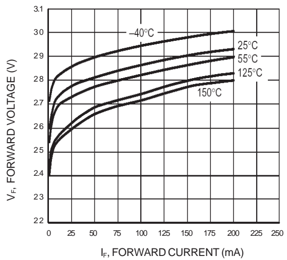
Figure 5. Forward Voltage
