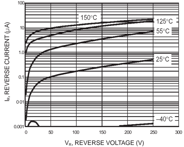
Figure 3. Leakage Current
