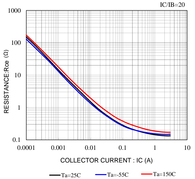
Fig.6 COLLECTOR-EMITTER SATURATION RESISTANCE VS.COLLECTOR CURRENT
