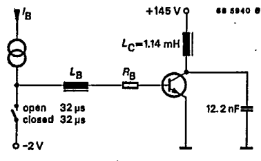
Test circuit for: t_s, t_f
