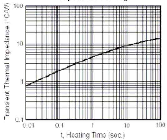
Fig. 6 -- Typical Transient Thermal Impedance Per Leg
