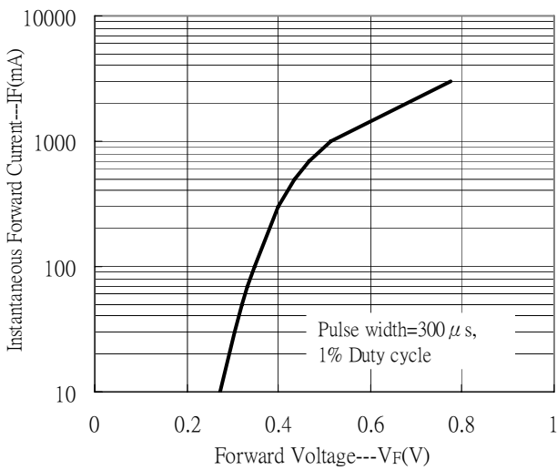
Fig. 3. Forward Characteristics
