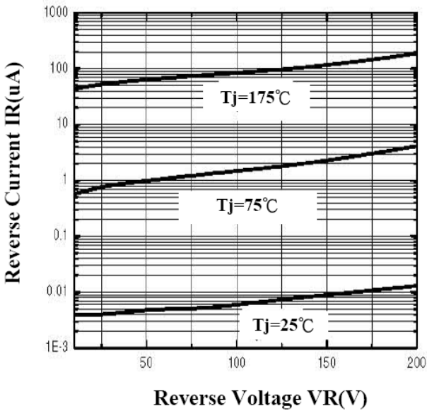
Fig.3- Typical Reverse
