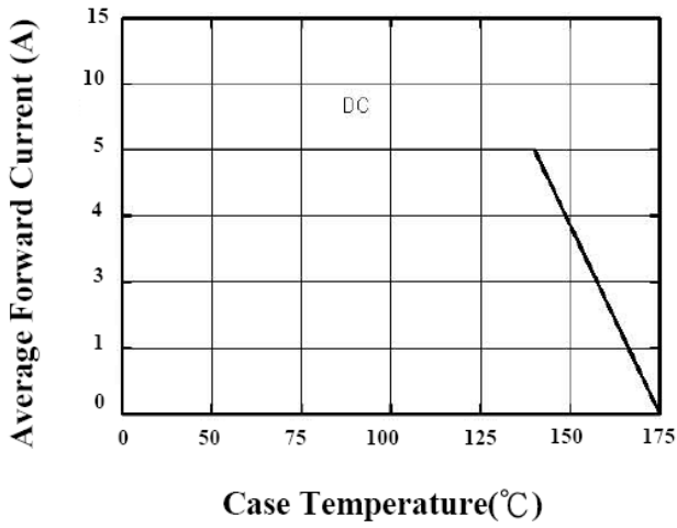
Fig.1- Forward Current
