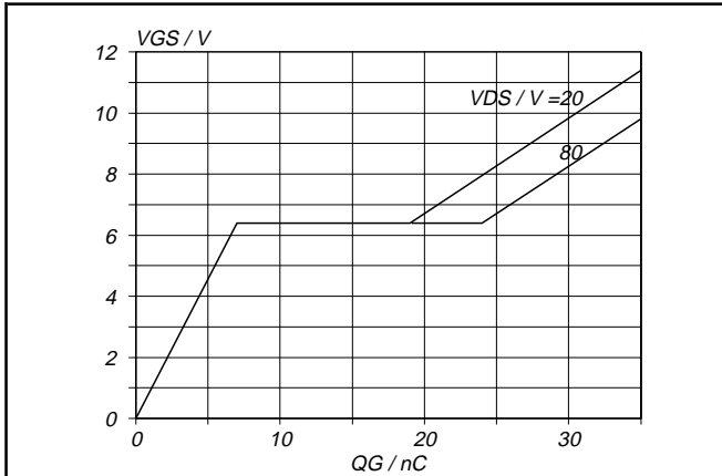
Fig.13. Typical turn-on gate-charge characteristics. V_{GS} = f(Q_G) ; conditions: I_D = 26\text{ A} ; parameter V_{DS}
