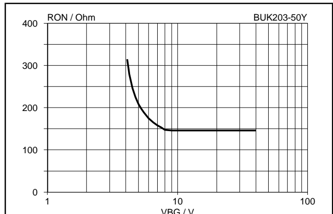
Fig.8. Typical on-state resistance, T_j = 25^\circ\text{C} . R_{ON} = f(V_{BG}) ; conditions: I_L = 2 \text{ A} ; t_p = 300 \mu\text{s}
