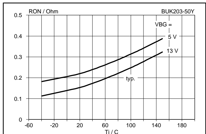
Fig.9. Typical on-state resistance, t_p = 300 \mu\text{s} . R_{ON} = f(T_j) ; parameter V_{BG} ; condition I_L = 0.5 \text{ A}
