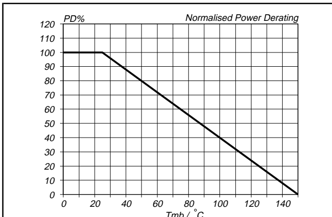
Fig.5. Normalised limiting power dissipation. P_D\% = 100 \cdot P_D / P_D(25\text{ }^\circ\text{C}) = f(T_{mb})
