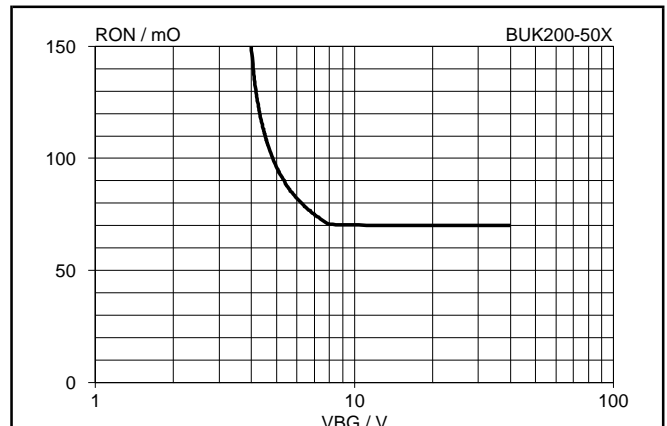
Fig.8. Typical on-state resistance, T_j = 25\text{ }^\circ\text{C} . R_{ON} = f(V_{BG}) ; conditions: I_L = 5\text{ A} ; t_p = 300\text{ }\mu\text{s}
