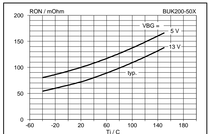
Fig.9. Typical on-state resistance, t_p = 300\text{ }\mu\text{s} . R_{ON} = f(T_j) ; parameter V_{BG} ; condition I_L = 1\text{ A}
