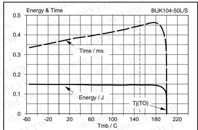
Fig.19. Typical overload protection characteristics. Conditions: V_{DD} = 13V ; V_{PS} = V_{PSN} ; V_{IS} = 7V ; SC load
