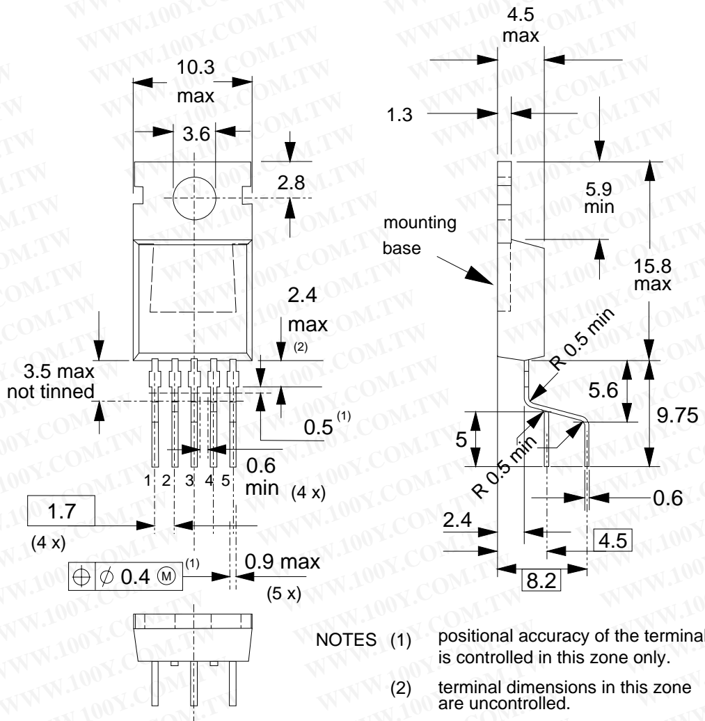
Fig.34. SOT263 leadform 263-01; pin 3 connected to mounting base.
