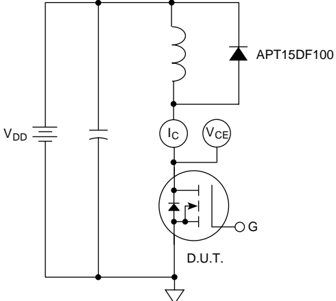
Figure 20, Inductive Switching Test Circuit
