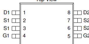
TSSOP-8 Top View
