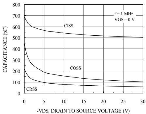
Figure 4. Capacitance Characteristics
