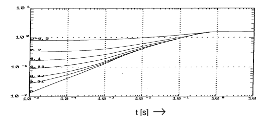
Z_{th(ch-c)} [K/W]
