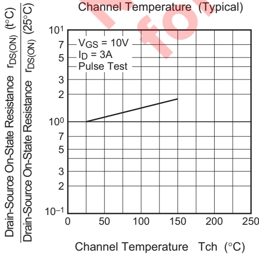
On-State Resistance vs. Channel Temperature (Typical)
