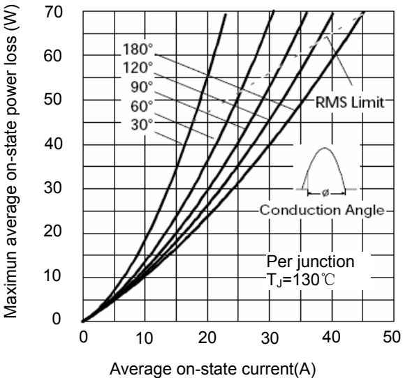
Figure 3. on-state power loss characteristics
