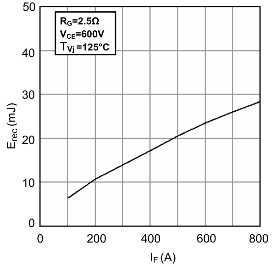
Figure8. Switching Energy vs. I_F
