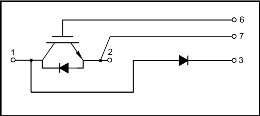
Figure11. Circuit Diagram
