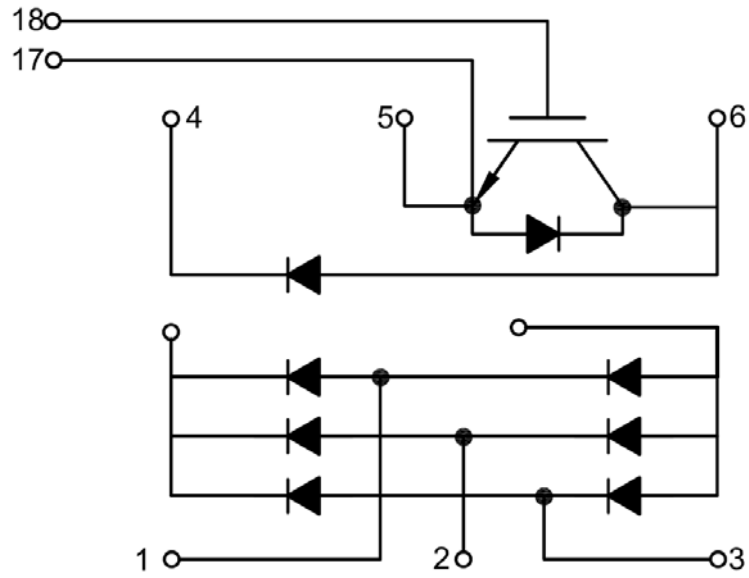
Figure14. Circuit Diagram
