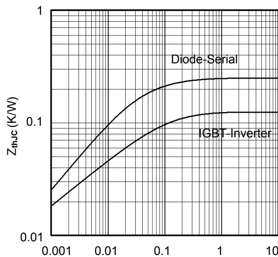
Rectangular Pulse Duration (seconds) Figure13. Transient Thermal Impedance
