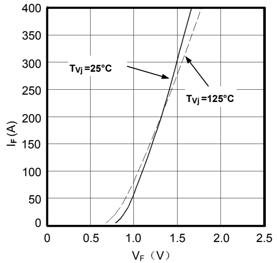
Figure12. Diode Forward Characteristics Rectifier -Diode
