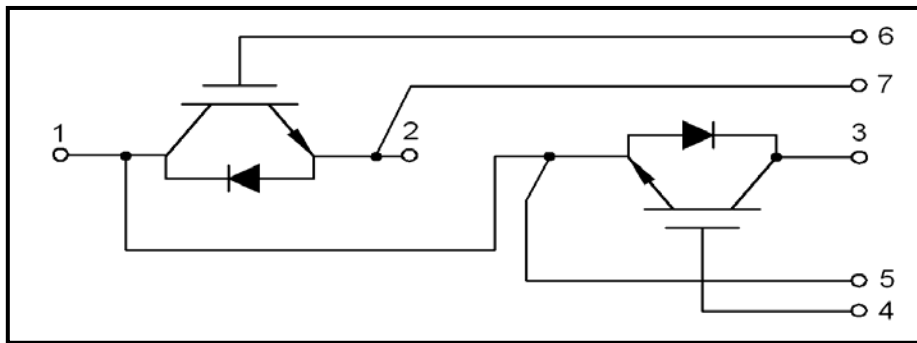
Figure11. Circuit Diagram
