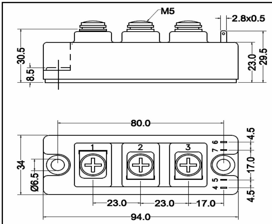
Dimensions (mm) Figure12. Package Outline
