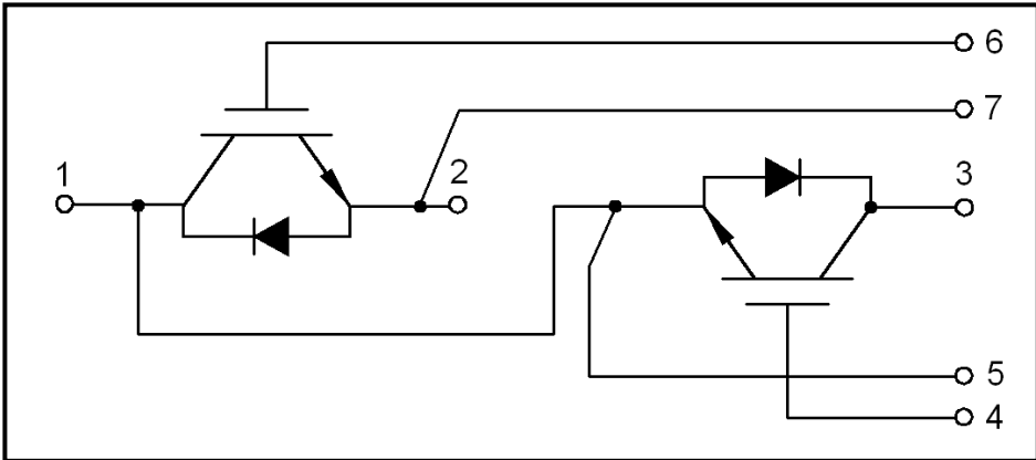
Figure11. Circuit Diagram
