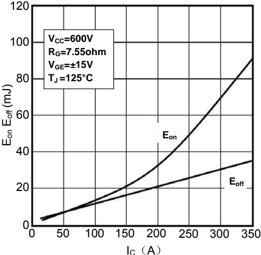
Figure3. Switching Energy vs. Collector Current
