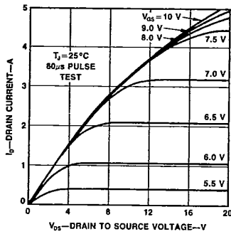
Figure 3 Output Characteristics
