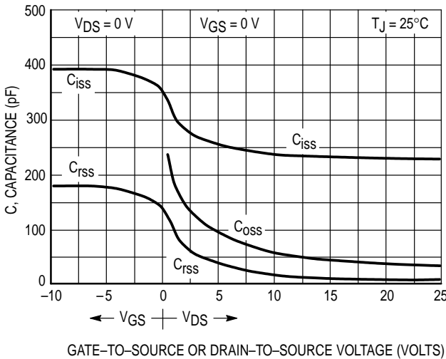
Figure 7a. Capacitance Variation
