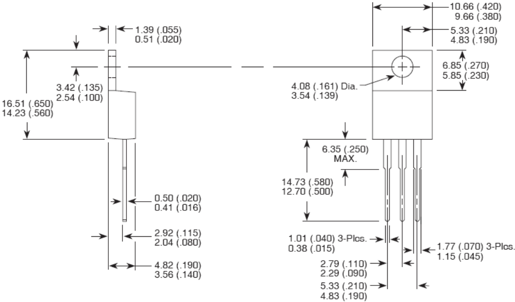
Dimensions in Millimeters and (Inchs) Fig8. Package Outline
