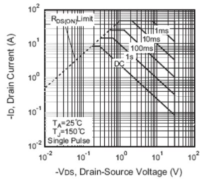
Figure 6. Maximum Safe Operating Area
