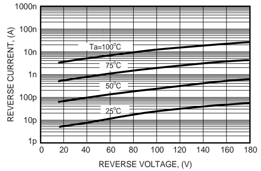
FIG. 2 - REVERSE CHARACTERISTICS
